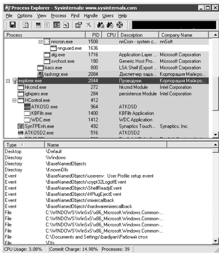
Рис. 9.6. Process Explorer
